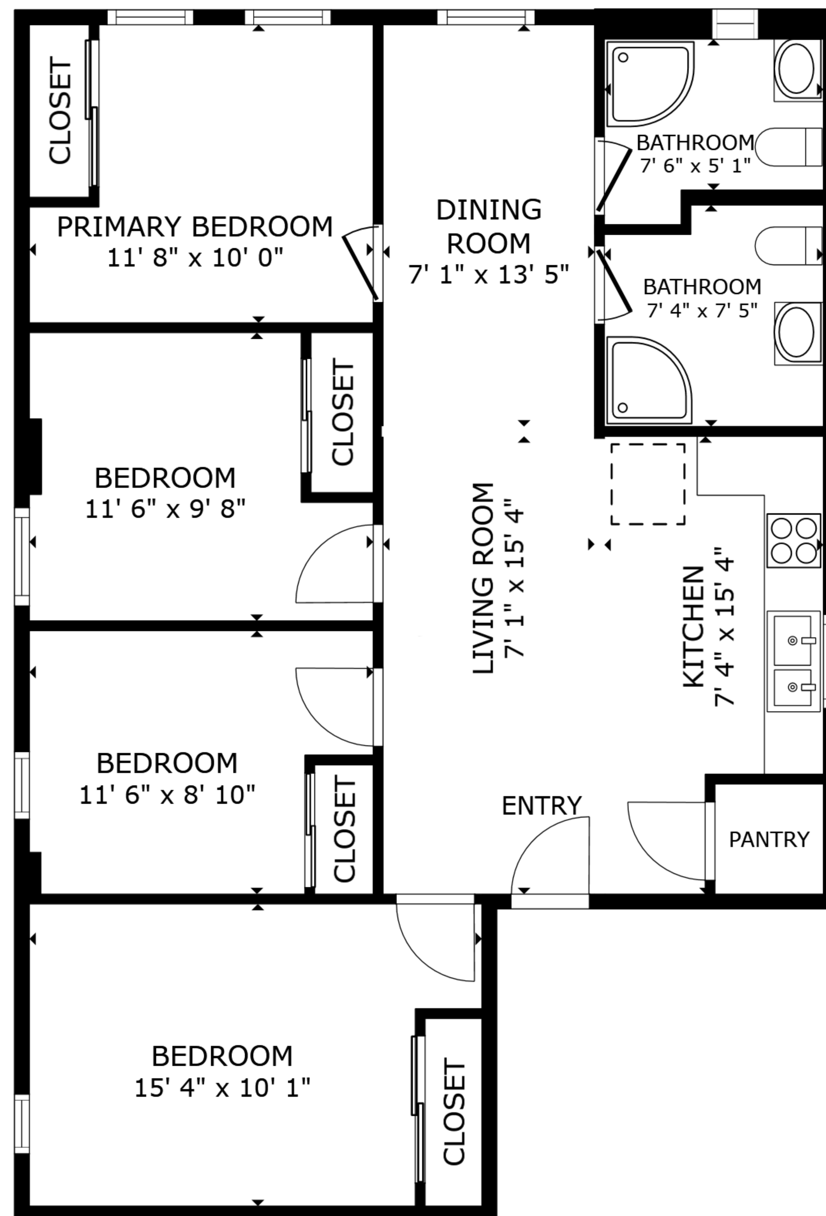
FLOOR PLAN
